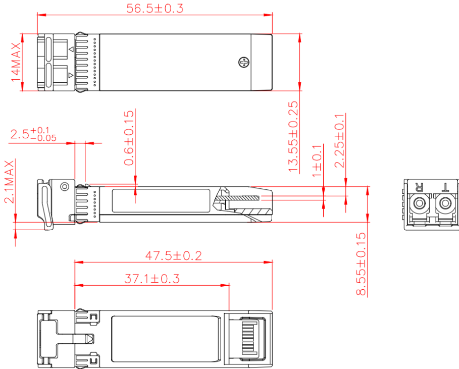
Figure 3. Module Mechanical Dimensions
