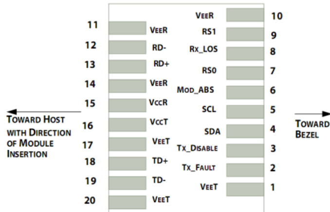
Figure 1.Pin function definitions
